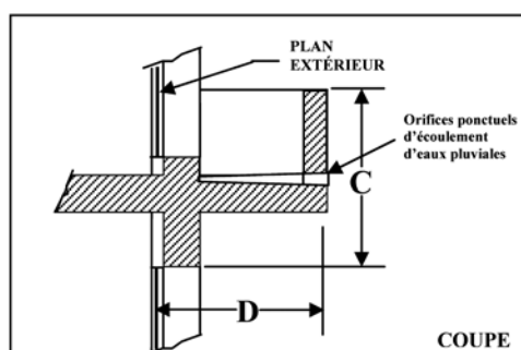
Figure A7 : garde-corps
